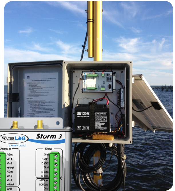
Example of a turn-key monitoring system containing a YSI Storm 3 Data Logger.
