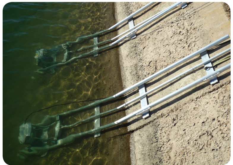
Example of a typical SonTek-SL1500 concrete lined canal installation as part of a HydroMet station.
