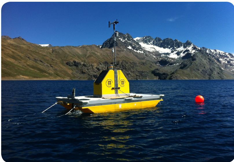
Monitoring Buoy containing a YSI Sonde, and meteorological sensors.
