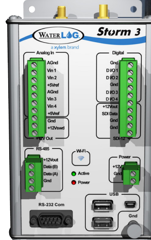
Example of a turn-key monitoring system containing a YSI Storm 3 Data Logger.
