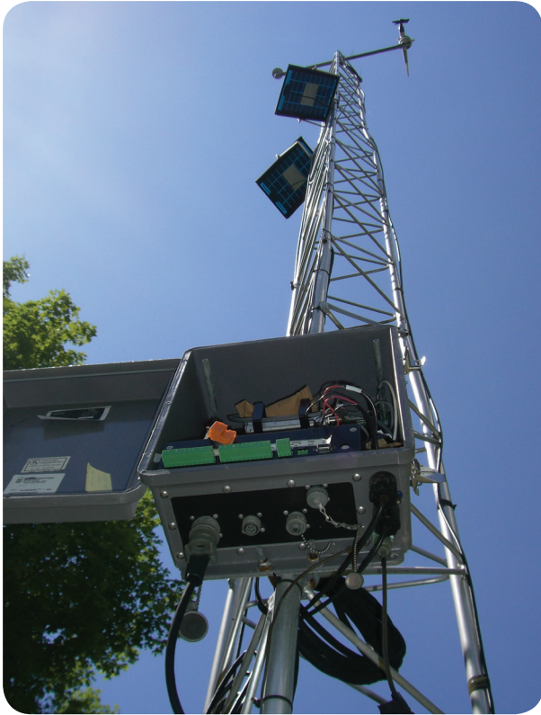
Monitoring tower containing a YSI Data Logger, and meteorological sensors
